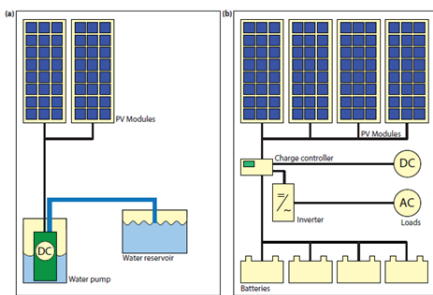
Gambar 1 Skema sistem PLTS off-grid
